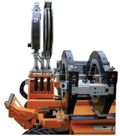
heating plate/facer disconnecting system
